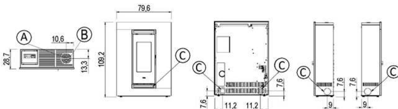
Fig. 23 - Luce Plus 7/9 UP-TWIN
