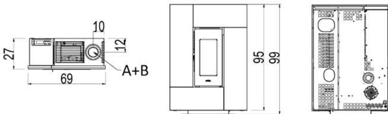
Fig. 24 - GRACE 7 UP-TWIN T2
