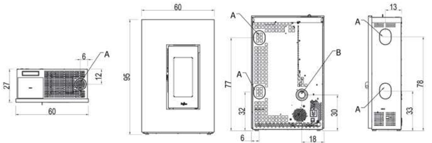
Fig. 28 - MADISON 5 T2 / SOLO 5 T2 / FLY 8 / XS7C
