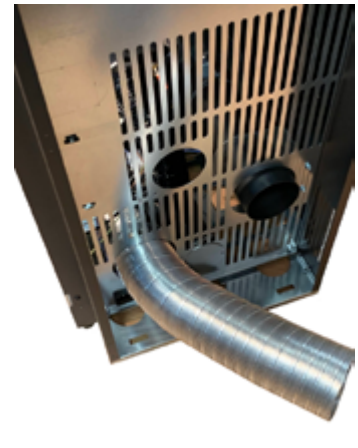
Fig. 74 - Raccorder le tuyau flexible
