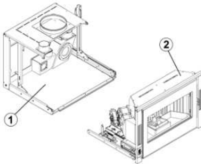
Fig. 27 - Structure + corps machine
