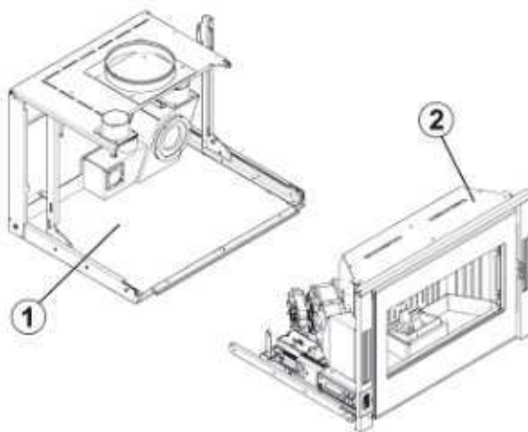
Fig. 27 - Structure + corps machine
